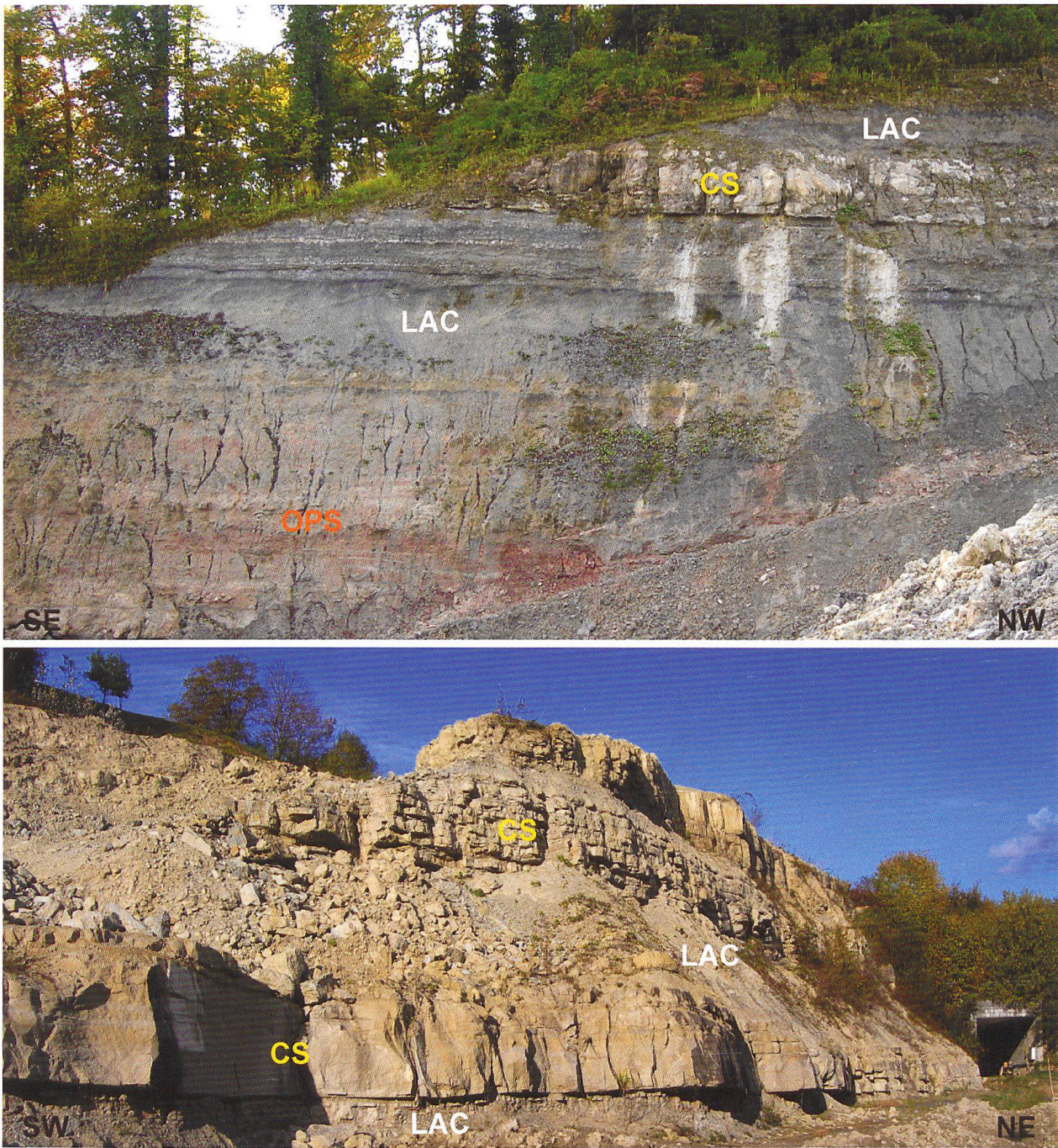
Fig. 18: Interpreted views of the marl pit Chörblige (Pfaffwil). Above: At the base with overbank fines and red palaeosols (OPS), grey lacustrine mudstones (LAC), blackish palaeosols and crevasse sands. Below: Lacustrine deposits (LAC) with low angle stratified crevasse splays and deltas (CS).
