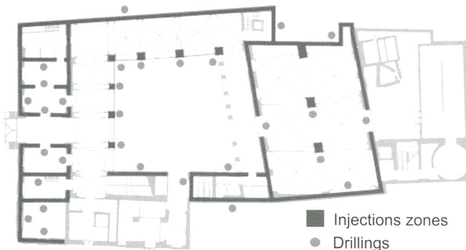
Fig. 2: Above: foundation survey at Palatium Vetus. Below: survey and intervention map.
