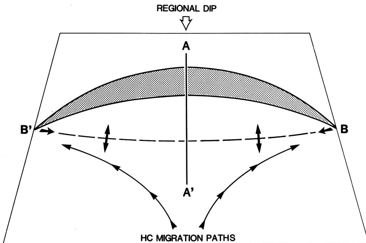
Figure 3: A simple growth-fault-scoop superimposed on regional dip in map view. Contrary to the thrust-fault-slipper the negative displacement on the growth fault produces an axial depression and not a culmination.
