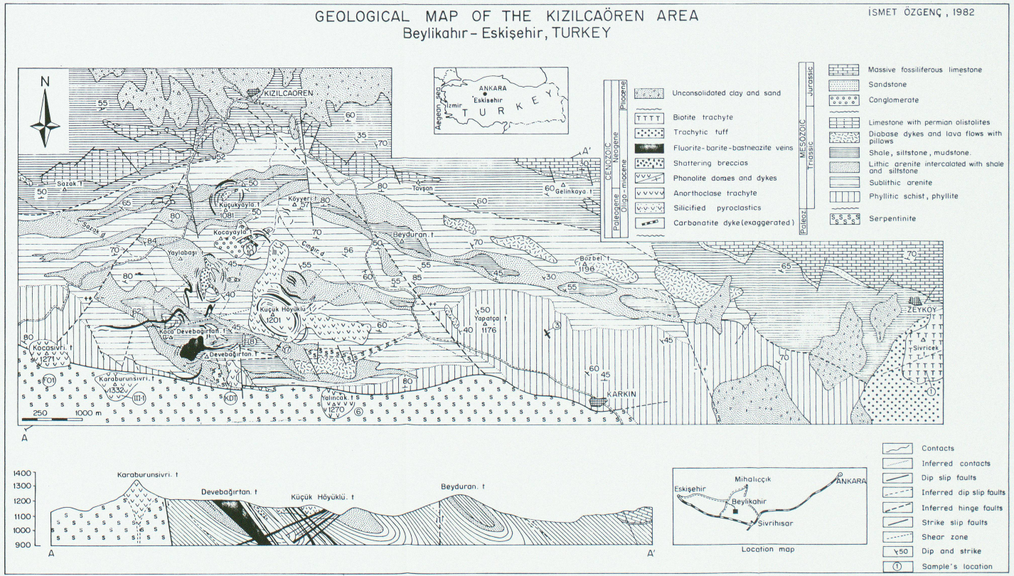
Fig. 1 Geological map of the Kızılcaören area with insets for location of the studied region.
