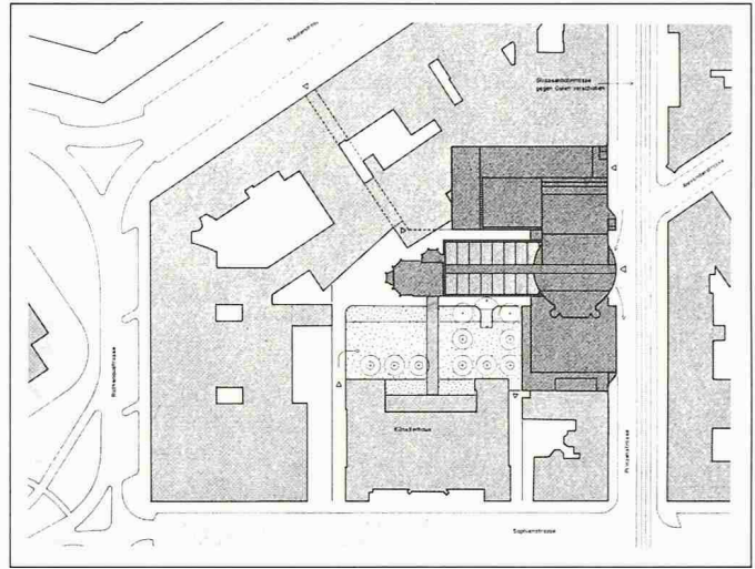
Situation 1:2600
