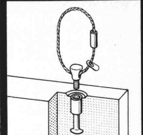
Tellerfuss-Anker
