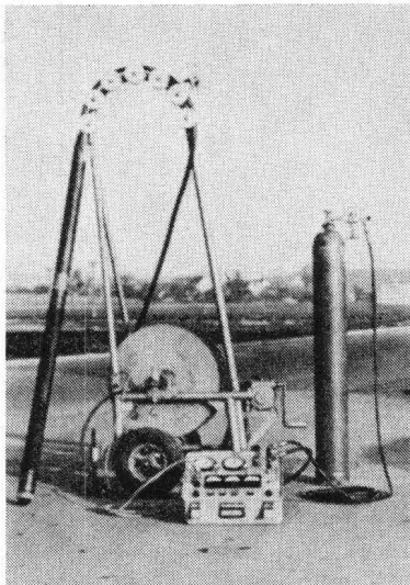
Dilatometer 95
