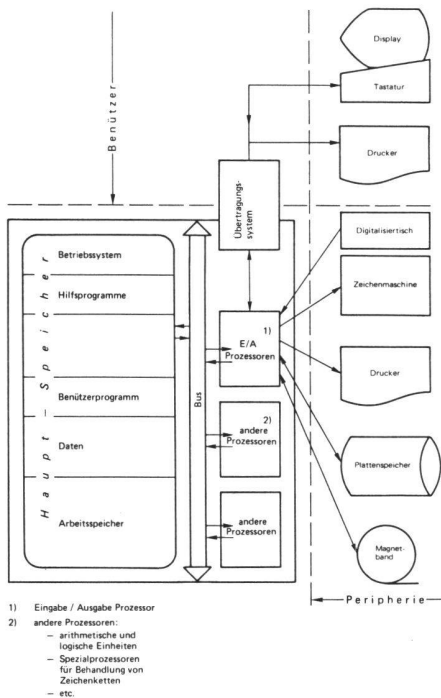
Abb. 4.1 Hardware-Schema
