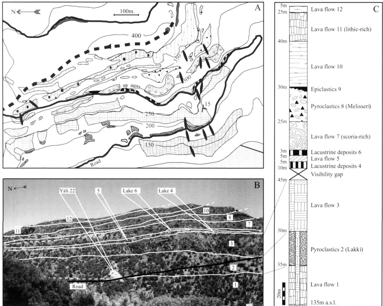
Fig. 5. Geological map (A) and photograph (B) of the caldera wall cut by the road from Mandraki. (C) General stratigraphy of the cliff. See legend in Fig. 2.
