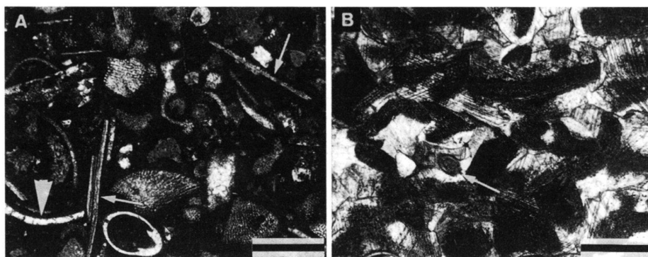
Fig. 9A. Crinoid-foraminifer packstone. Fragments of crinoids, benthic foraminifers (bottom center), Entolium fragments (arrows), and molluscs other than Entolium (arrowhead) in a micritic matrix. Sample Zn. 9. Cortijo del Zegrí. Scale bar = 500 µm. B. Crinoid grainstone. Crinoid fragments and some benthic foraminifers (arrow) cemented by syntaxial calcite growing from crinoid ossicles. Sample Zn. 22. Cortijo del Zegrí. Scale bar = 500 µm.
