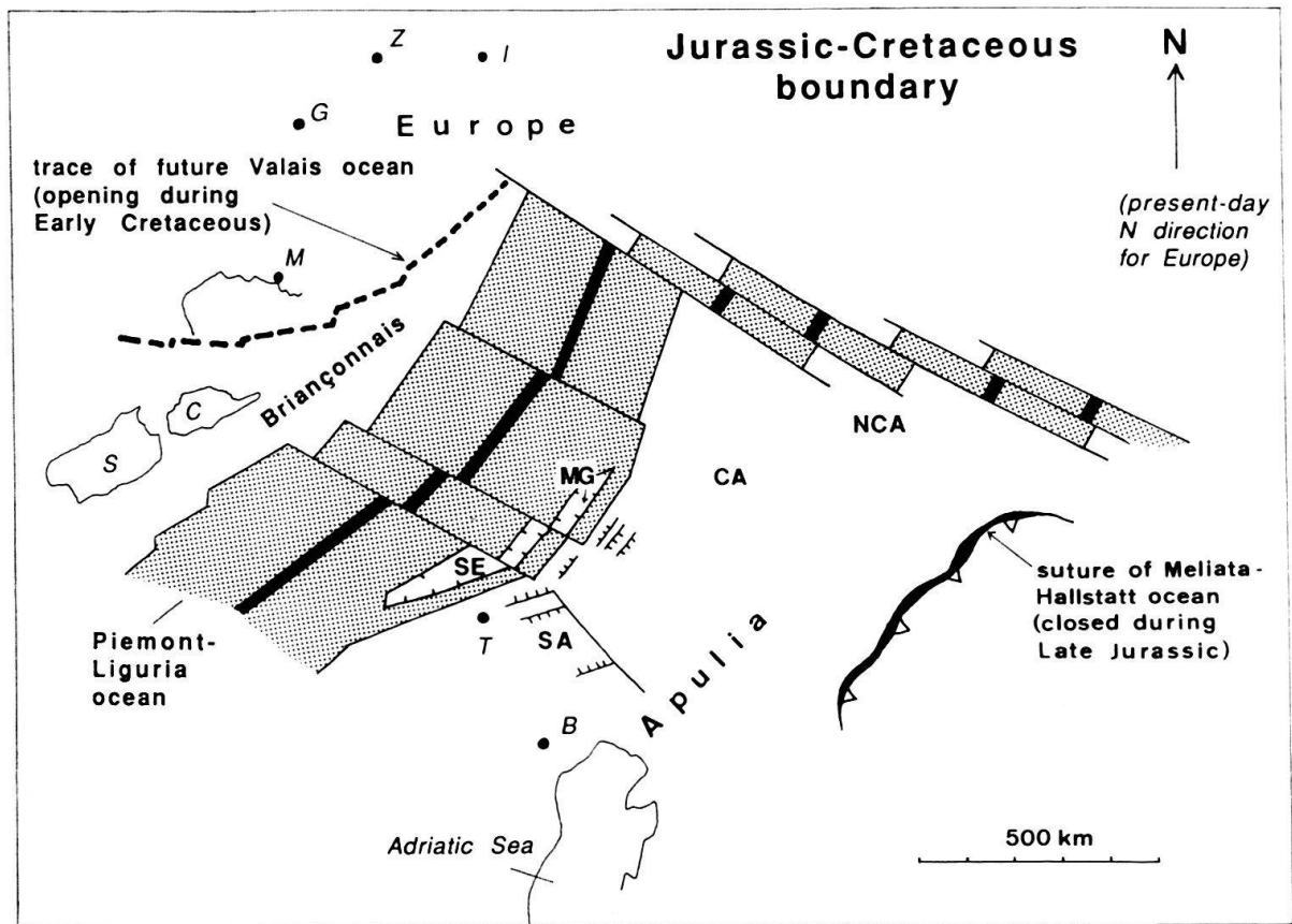
Fig. 2. Paleogeography in the Alpine realm reconstructed for the Jurassic-Cretaceous boundary time. CA, Central Austroalpine; MG, Margna; NCA, Northern Calcareous Alps; SA, Southern Alps; SE, Sesia; B, Bologna; C, Corsica; G, Geneva; I, Innsbruck; M, Marseille; S, Sardinia; T, Torino; Z, Zürich. After Dercourt et al. (1986), Stampfli (1993), and Schmid et al. (in press a).
