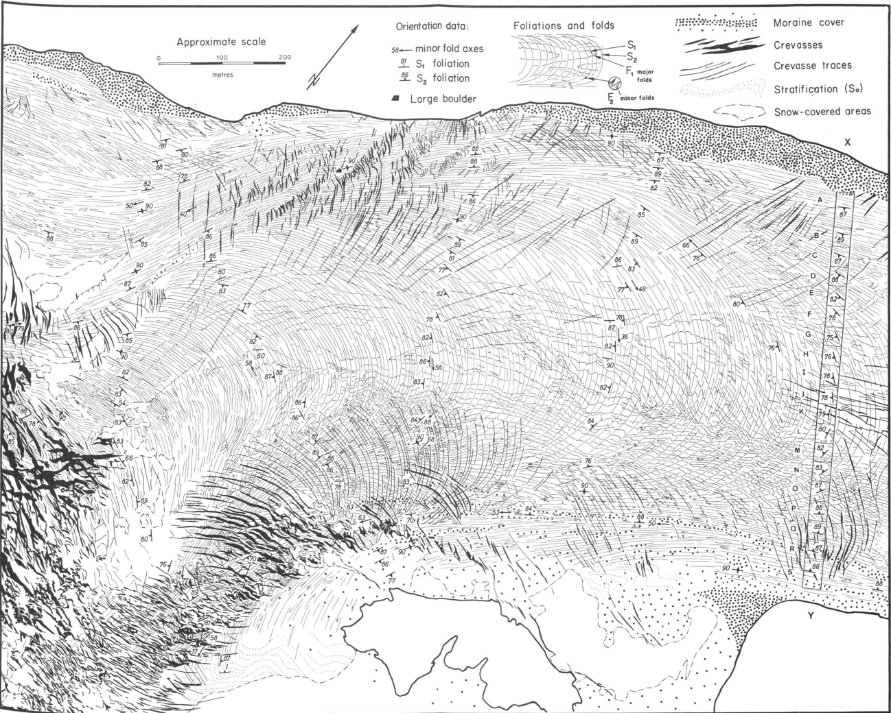
Structural relations in the Bättelmatthorn sector of Griesgletscher (Valais, Switzerland) based on a vertical aerial photograph taken on 6 September 1973.
