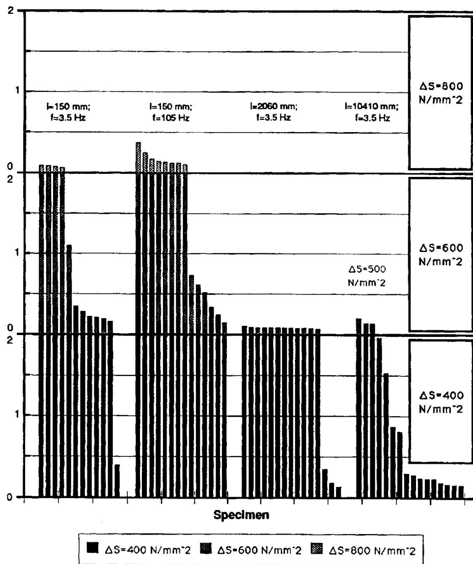
Fig. 3: Summary of fatigue test results on prestressing wires for different proof length
