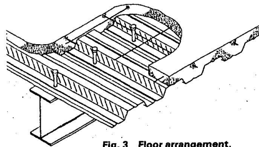
Fig. 3 Floor arrangement.
