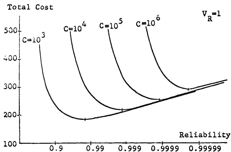
FIG. 1 TOTAL COST VS. ELEMENT RELIABILITY-- SERIES SYSTEM
