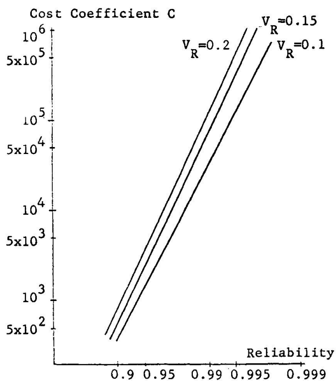
FIG. 3 COST COEFFICIENT VS. OPTIMAL ELEMENT RELIABILITY-- PARALLEL SYSTEM
