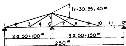
Fig. 8 2 Span Model
