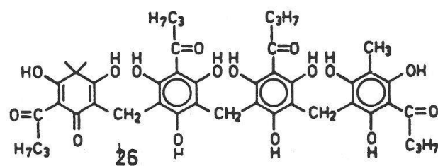
Tetraflavaspidic acid - BBBB
