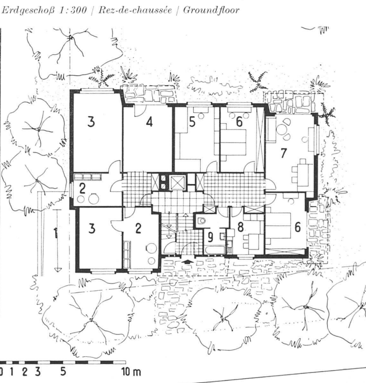
Erdgeschoß 1:300 | Rez-de-chaussée | Ground floor
