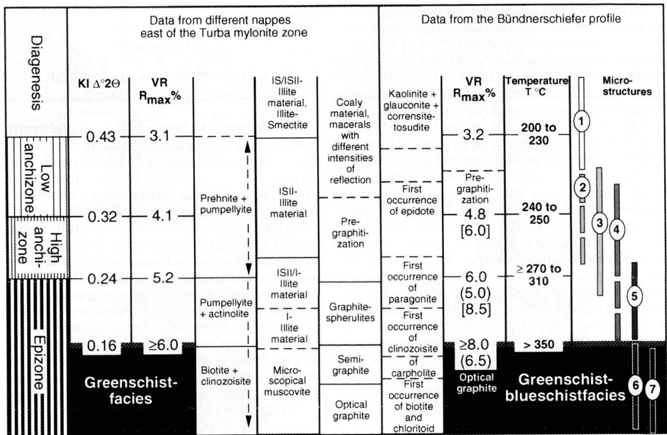
Fig. 5 Comparison of metamorphic data from east of the "Turba mylonite zone" (NIEVERGELT et al., 1996) and this study. The mineral data, vitrinite reflectance (VR) and temperature estimations are taken from OBERHÄNSLI et al. (1995), FREY and FERREIRO MÄHLMANN (1999), and PETROVA et al. (2002). Data from different nappes east of the Turba mylonite zone are compiled from FERREIRO MÄHLMANN (1996, 2001). I—illite, S—smectite, KI—illite crystallinity shown as Kübler Index. Values in parenthesis give the correlation from the areas of blueschist facies overprint. Values in brackets give the correlation from shear zones. The occurrence of microstructures is shown in the last column: 1—amorphous carbon, 2—initial onions (range not well constrained), 3—different types of carbon onions, 4—onions with thickened rims (lower range limit not well constrained), 5—polygonal onions, 6—broken onions, 7—graphite flakes.
