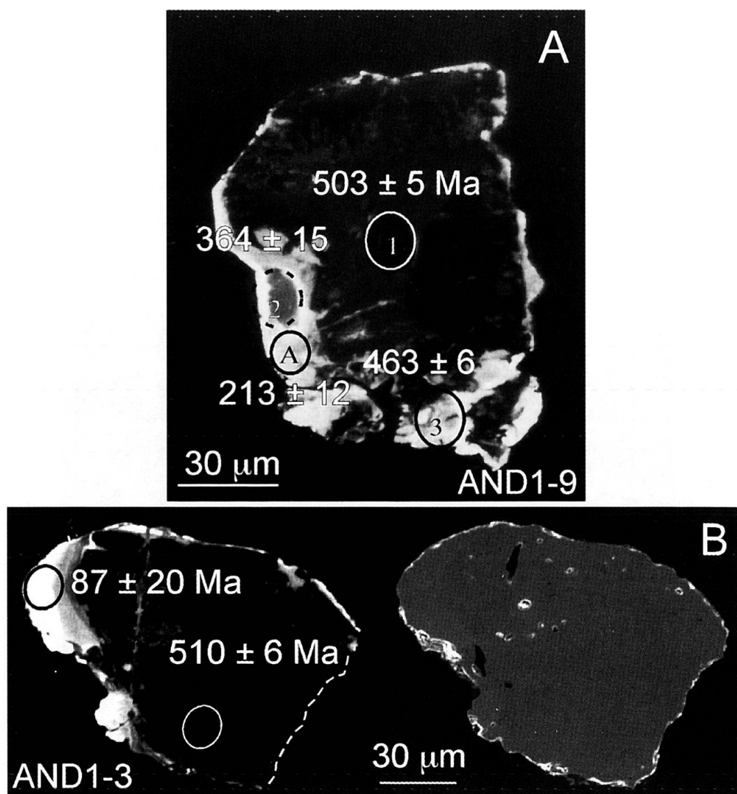
Fig. 3 Cathodoluminescence (CL) pictures (A and left side in B) and secondary electron (SE) pictures (right side in B) of co-magmatic zircon crystals from the amphibolitized eclogite of Andolla. In (A) note that the pit generated during SHRIMP analysis (Nr. 2) shows weak CL (dark appearance), which is interpreted to be due to the presence of an underlying magmatic core (see text). In (B) note the two distinct metamorphic rims (inner darker and outer lighter in CL) formed by recrystallization probably during different stages of metamorphism or during different metamorphic episodes (see also text).
