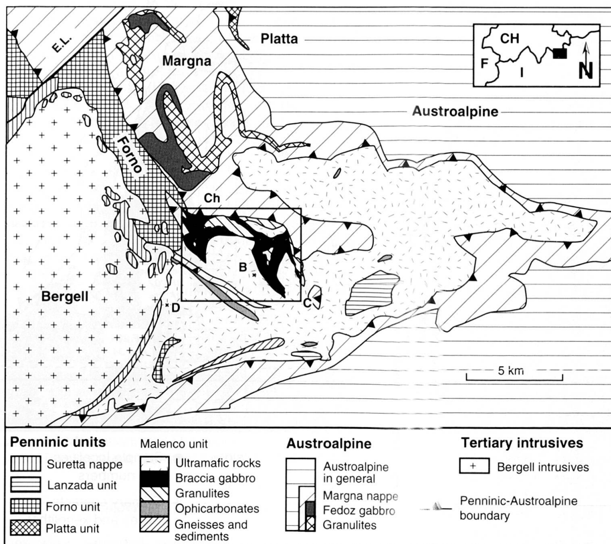
Fig. 1 Tectonic map of the Penninic-Austroalpine boundary in Val Malenco (N Italy), modified from MÜNTNER and HERMANN (1996). The inset in the upper right corner shows the geographic position of this area at the Swiss-Italian border zone. The frame outlines the study area which is shown in more detail in figure 2. B = Monte Braccia, D = Monte Disgrazia, C = Chiesa, Ch = Chiareggio, E.L. = Engadine Line.
