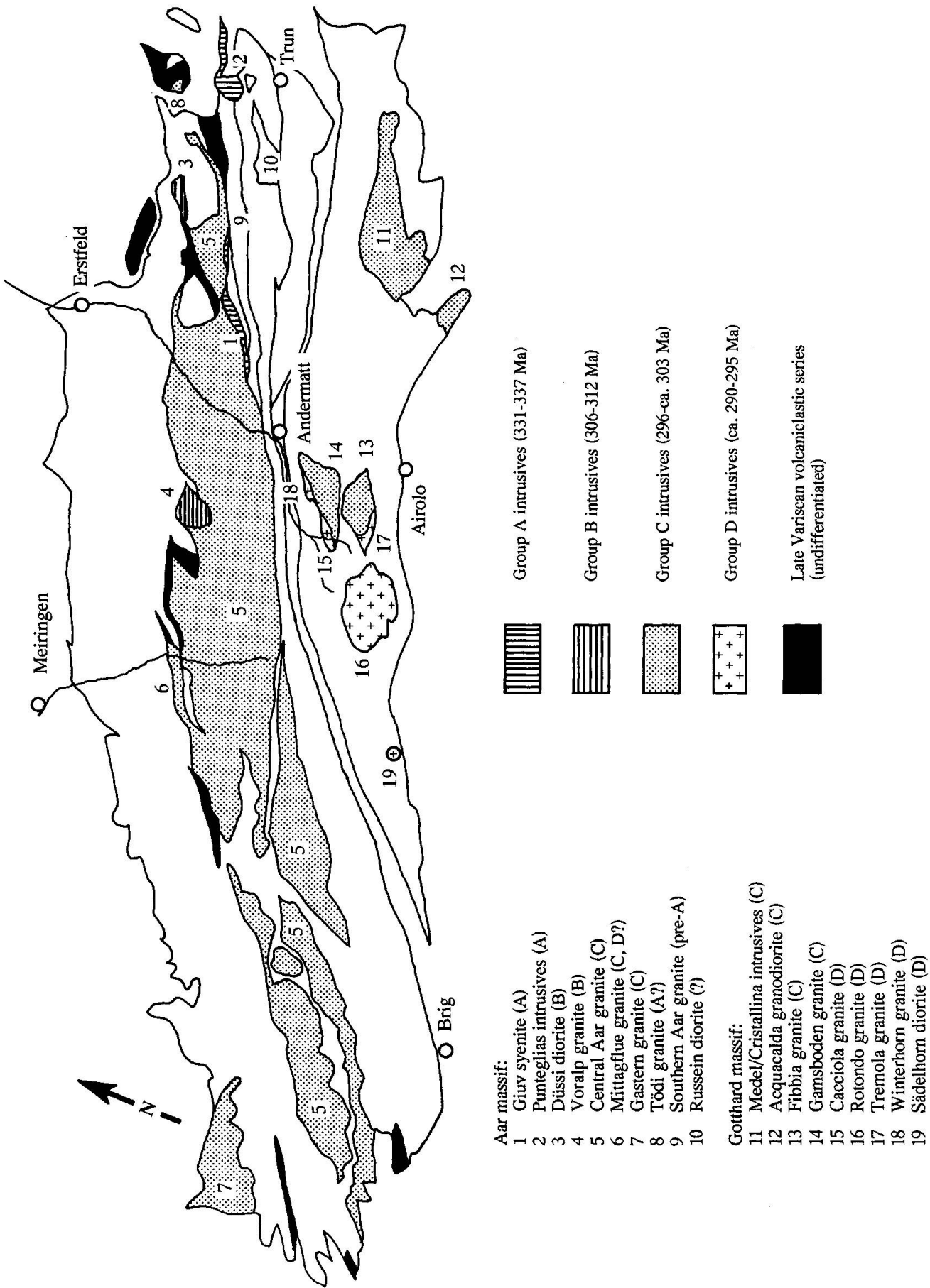
Fig. 1 Schematic map of the Aar and Gotthard massifs with the sequence of late Variscan magmatic rocks.
