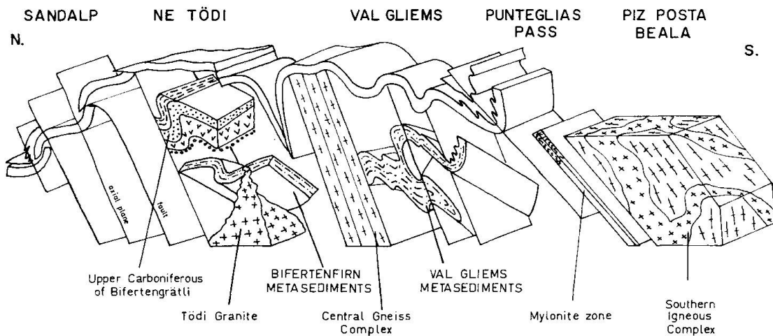
Fig. 2. Schematic block diagram of the pre-Triassic sediments and folding of the Triassic unconformity in the Tödi area. (Triassic Röti Dolomite indicated as the folded layer above the unconformity.)
