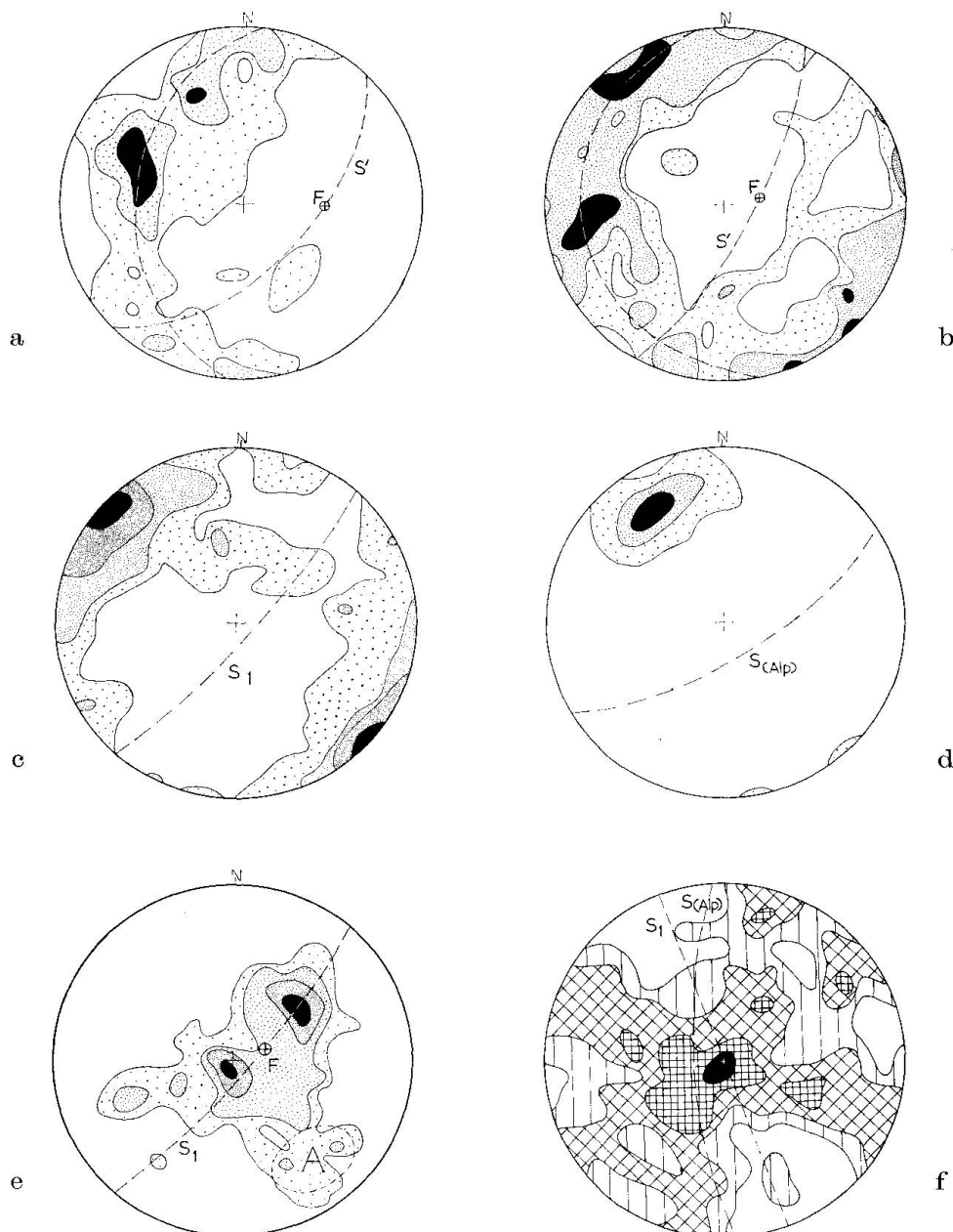
Fig. 14. Measurements of structural elements of the Bifertenfirn and Val Gliems metasediments: Lambert's projection, lower hemisphere. a, \pi -diagram (108 poles to bedding) of the Bifertenfirn metasediments. Contours 5%, 3%, 1% per 1% area. b, \pi -diagram of the pre-Triassic sediments of Val Gliems, 133 poles. Contours 5%, 2%, 1% per 1% area. F = constructed fold axis. c, Poles to pre-Alpine cleavage in the Val Gliems metasediments; 225 poles. Contours 20%, 10%, 5%, 1% per 1% area. S_1 = general cleavage plane. d, 70 poles to Alpine cleavage in Val Gliems; contours 15%, 7%, 1% per 1% area. e, Elongation directions in the Val Gliems metasediments, 74 point. Contours 10%, 7.5%, 3%, 1% per 1% area. S_1 = pre-Alpine cleavage plane; F = constructed fold axis from \pi -diagram; A = field of Alpine lineation. f, Orientation diagram for (0001) of quartz in quartzite pebble in conglomerates, Val Gliems, 362 grains. Contours 5%, 2%, 1.2%, 0.75% per 1% area.
