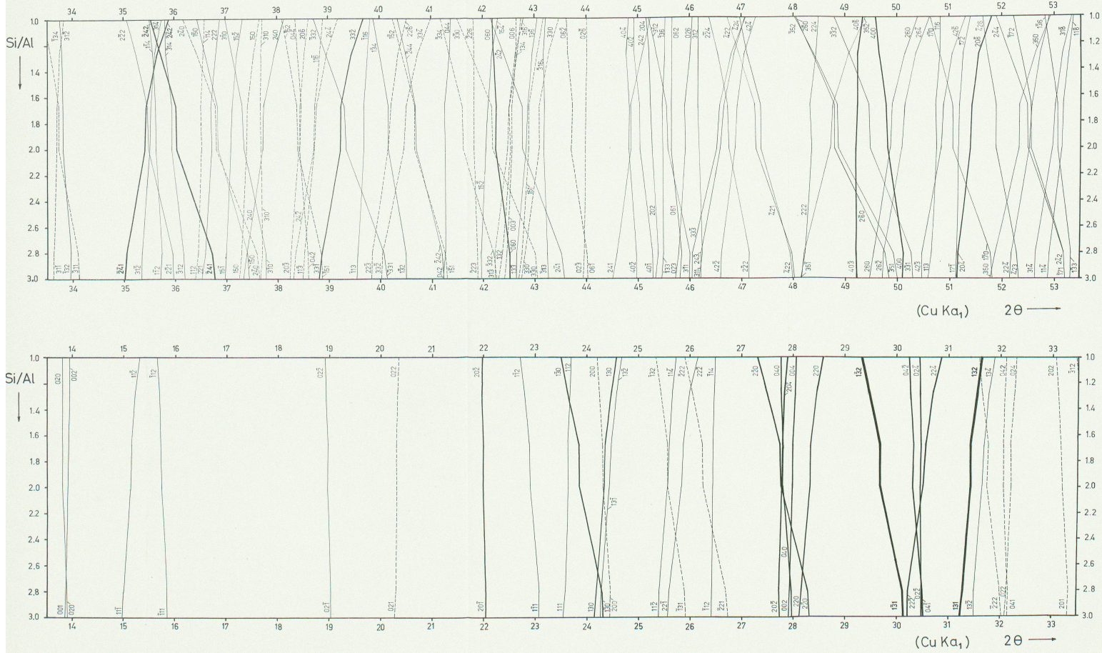
Fig. 1. Relations between 2θ (Cu Kα 1 ) and chemical composition (given as Si/Al-ratio) in the powder patterns of "plagioclase (low)".
