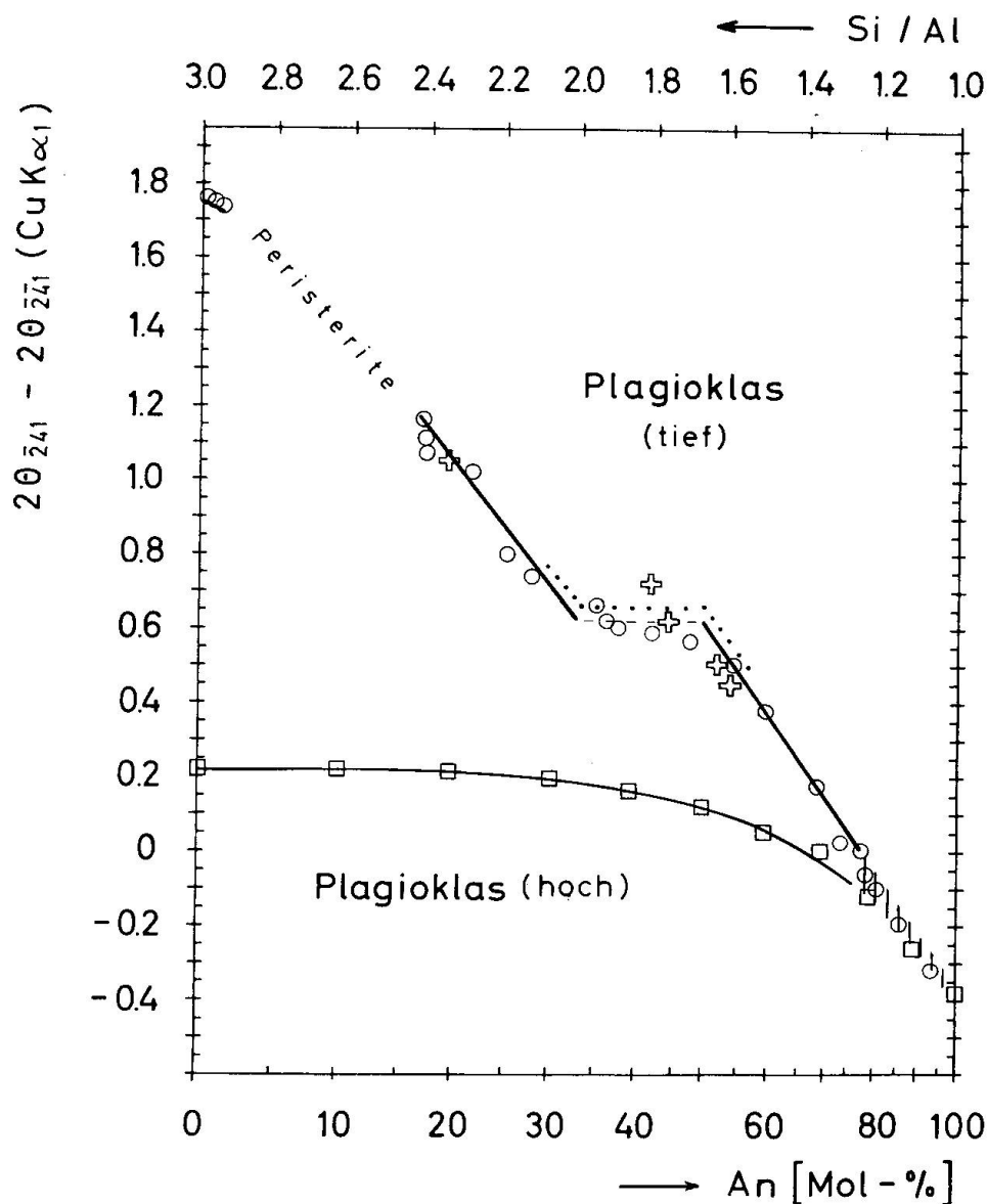
Fig. 6. Boundary curves for the variation of \Delta(\theta)_2 = 2\bar{\theta}_{241} - 2\bar{\theta}_{2\bar{4}1} (Cu K\alpha_1 radiation) and Si/Al ratio (An content also shown) for plagioclases with Or < 0.5-0.8 . The dotted boundary curve is for "plagioclase (low)" with ca. An_{40-60} and Or_4 . \circ , "plagioclase (low)", Or < 0.5-0.8 ; \square , synthetic "plagioclase (high)"; \oplus , "plagioclase (low)", Or_{ca. 4} .
