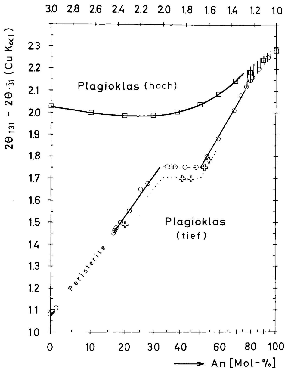
Fig. 5. Boundary curves for the variation of \Delta(\theta)_1 = 2\theta_{131} - 2\theta_{1\bar{3}1} (Cu K \alpha_1 radiation) and Si/Al ratio (An content also shown) for plagioclases with Or _{<0.5-0.8} . The dotted boundary curve is for "plagioclase (low)" with ca. An _{40-60} and Or _4 . \circ , "plagioclase (low)", Or _{<0.5-0.8} ; \square , synthetic "plagioclase (high)"; \oplus , "plagioclase (low)", Or _{ca. 4} .
