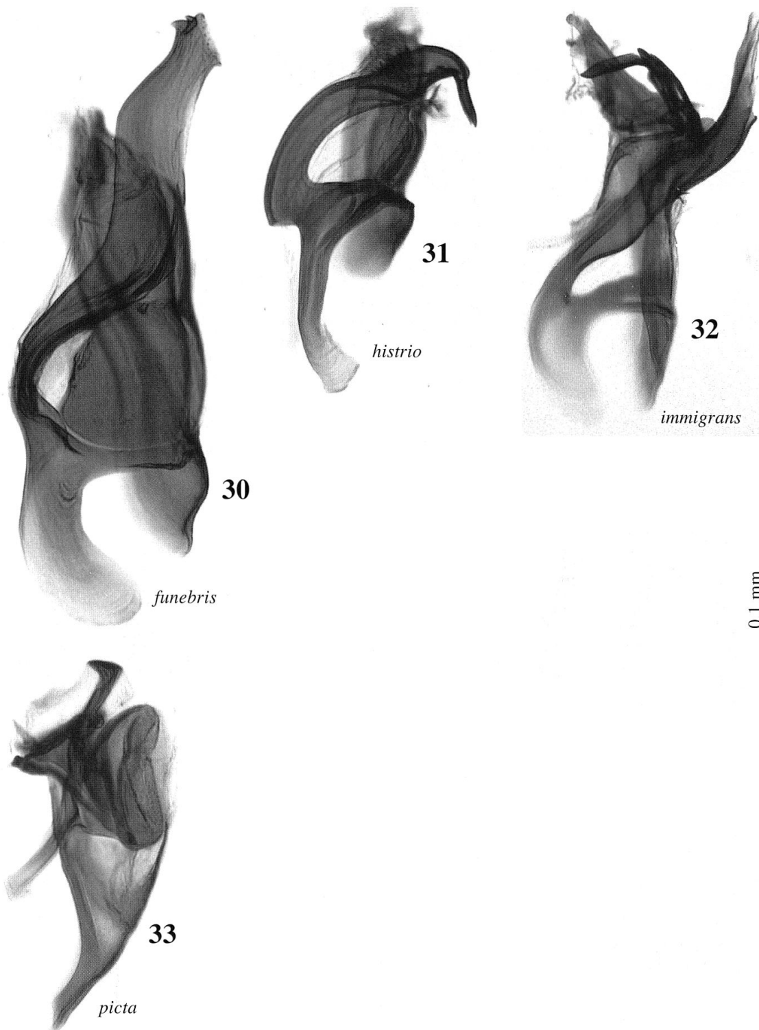
Figs 30–33. Photomicrographs of internal male terminalia of Drosophila species, left lateral view. 30: D. funebis , Seelisberg, Switzerland; 31: D. histrion , Rheineck, Switzerland; 32: D. immigrans , Gomel, Belarus; 33: D. picta , Bordils, Spain.
