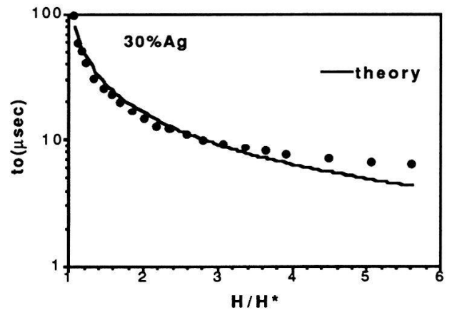
Fig. 3 Experimental and theoretical values of t_0 Vs H/H^* for x = 0.3 .
