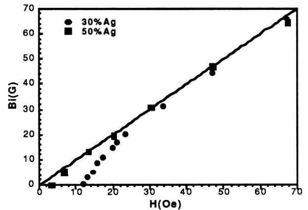
Fig. 2 Bi-H curves for samples containing 30% and 50% Ag.
