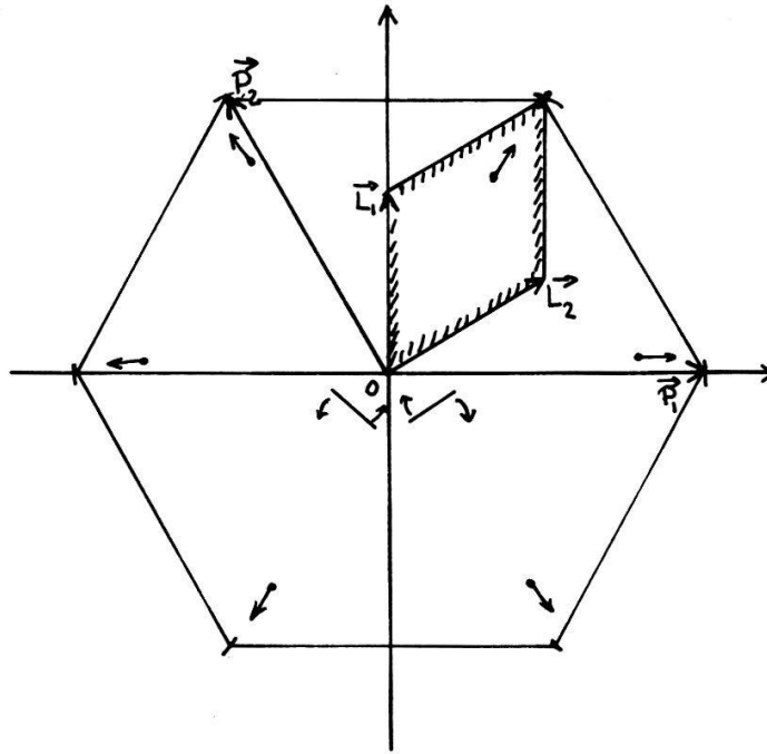
Fig. 7 The Frenkel-Kac construction for the group SU(3)
