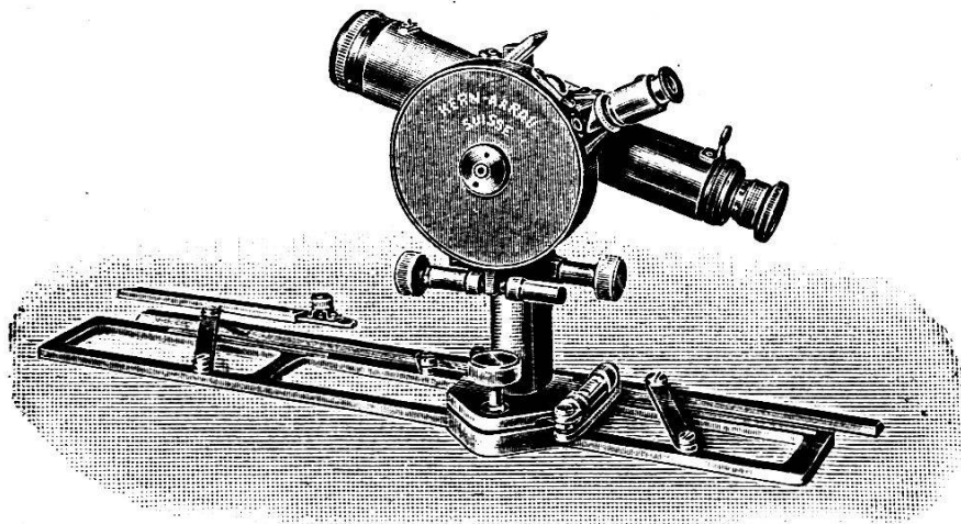
Kippregel No. 76
