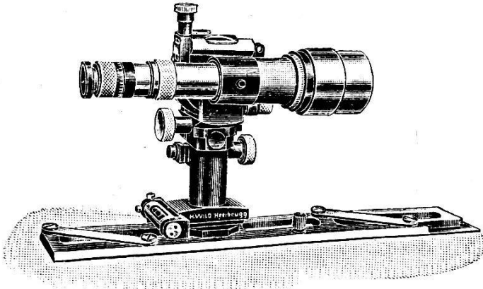
Kippregel Wild
