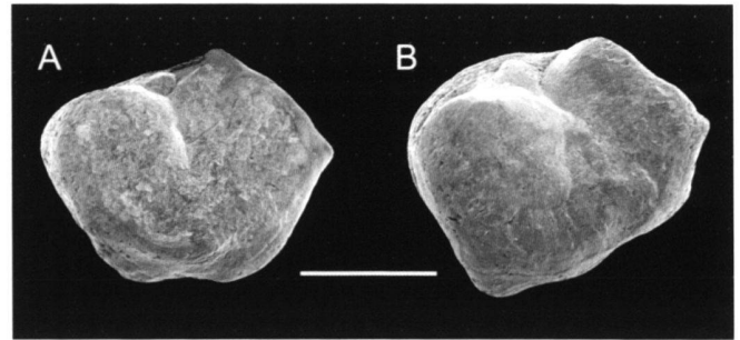
Fig. 6. Palaeotınca sp. otoliths (left lapilli), Upper Marine Molasse (Karpatian), Mauensee, central Switzerland. A, B) Dorsal view, mirrored (BSPG 2003 XVIII 90–91). SEM pictures. Scale bar: 0.5 mm.
