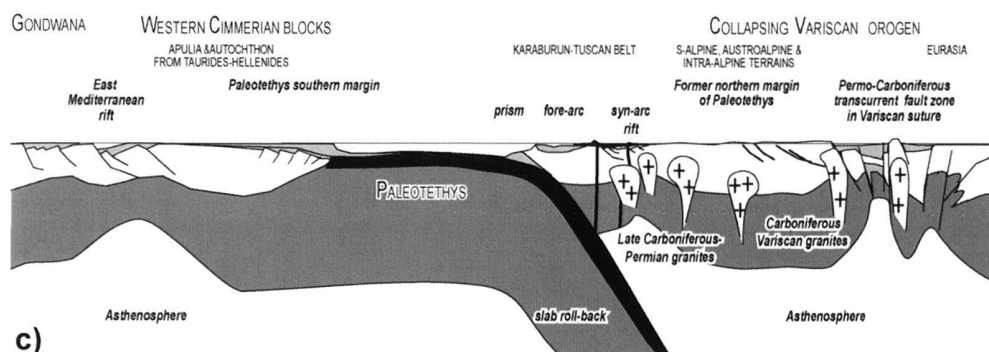
Fig. 18. Paleotectonic reconstructions in the Mediterranean area (Stampfli et al. 2003). a) Sakmarian map (280 My); b) Late Carnian (220 My); c) Late Permian cross-section located in a). A star locates the studied area in a) and b). AA: Austroalpine east; Ab: Alboran; Ad: Adria; Am: Armorica; An: Antalya; Ap: Apulia s.str.; Aq: Aquitain; Bd: Beydaglari; Br: Briançonnais; Bü: Bükk, Fatric; Ce: Cetic; Ch: Channel; Cn: Carnic; Ct: Cantabria; CP: Calabria, Peloritani; Cv: Canavese; DH: Dinaro-Hellenic; Do: Dobrogea; He: Helvetic rim basin; Hk: high karst; Ib: Iberia central; Ig: Igal; Is: Istanbul; Kb: Karaburun; Kk: Karakaya; KS: Kotel-Strandja; La: Lagonegro; Lg: Ligerian; Ma: Mani; MD: Moldanubian; Mg: Magura; MM: Meseta Morocco; Mn: Menderes; Mo: Moesia; Mr: Mrzlevodice fore-arc; Mz: Munzur; OM: Ossa-Morena; PD: Pindos; Pe: Penninic; Pl: Pelagonian; Rh: Rhodope; RH: Rheno-Hercynian; sA: southern Alps; Sb: sub-Betic rim basin; Se: Sesia, Austroalpine west; Si: Sicilian basin; Sk: Sakarya; SM: Serbo-Macedonian; SS: Sanandaj-Sirjan; St: Sitia; Sx: Saxothuringian; Ta: West-Taurus; TD: Trans-Danubian range; To: Taleo Ori; Tt: Tatic; Tu: Tuscan nappes; Ty: Tyros; Tz: Apuseni, Tizia; wC: western Crete; WC: Western Carpathian; Zo: Zonguldak.
