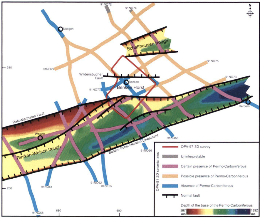
Fig. 9. Isochron map of the BPC horizon where the presence of PC deposits is considered as certain. Along some of the 2D seismic line segments, extending beyond the area of the established PC graben, some weak indications suggest the possible presence of PC deposits.
