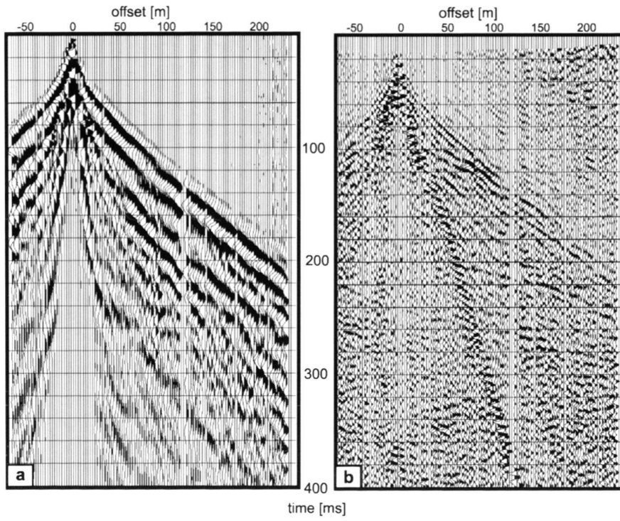
Fig. 4. Example of a shot gather of (a) raw data with only trace equalisation applied, and (b) the same data after applying initial processing including amplitude scaling, refraction static correction, spectral whitening, and frequency filtering.
