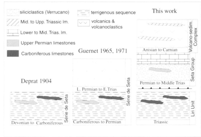
Fig. 2. Pre Norian Units of central Evia: old and new stratigraphic subdivisions.
