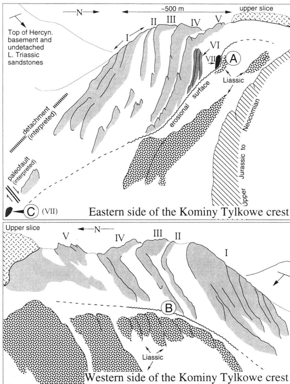
Fig. 5. Interpreted photographs of an inverted Lower Liassic erosional unconformity corresponding to the rift-onset unconformity on both sides of the Kominy Tylkowie crest (location Fig. 2). Roman-type numbers refer to Triassic limestone marker beds (shaded; see Fig. 3) which are truncated by the erosional surface. According to our interpretation, spots A, B and C, also shown on Fig. 6, refer to the upper part of the footwall block, to the lower part of the footwall block, and to the hangingwall block respectively (see Fig. 6, right part).
