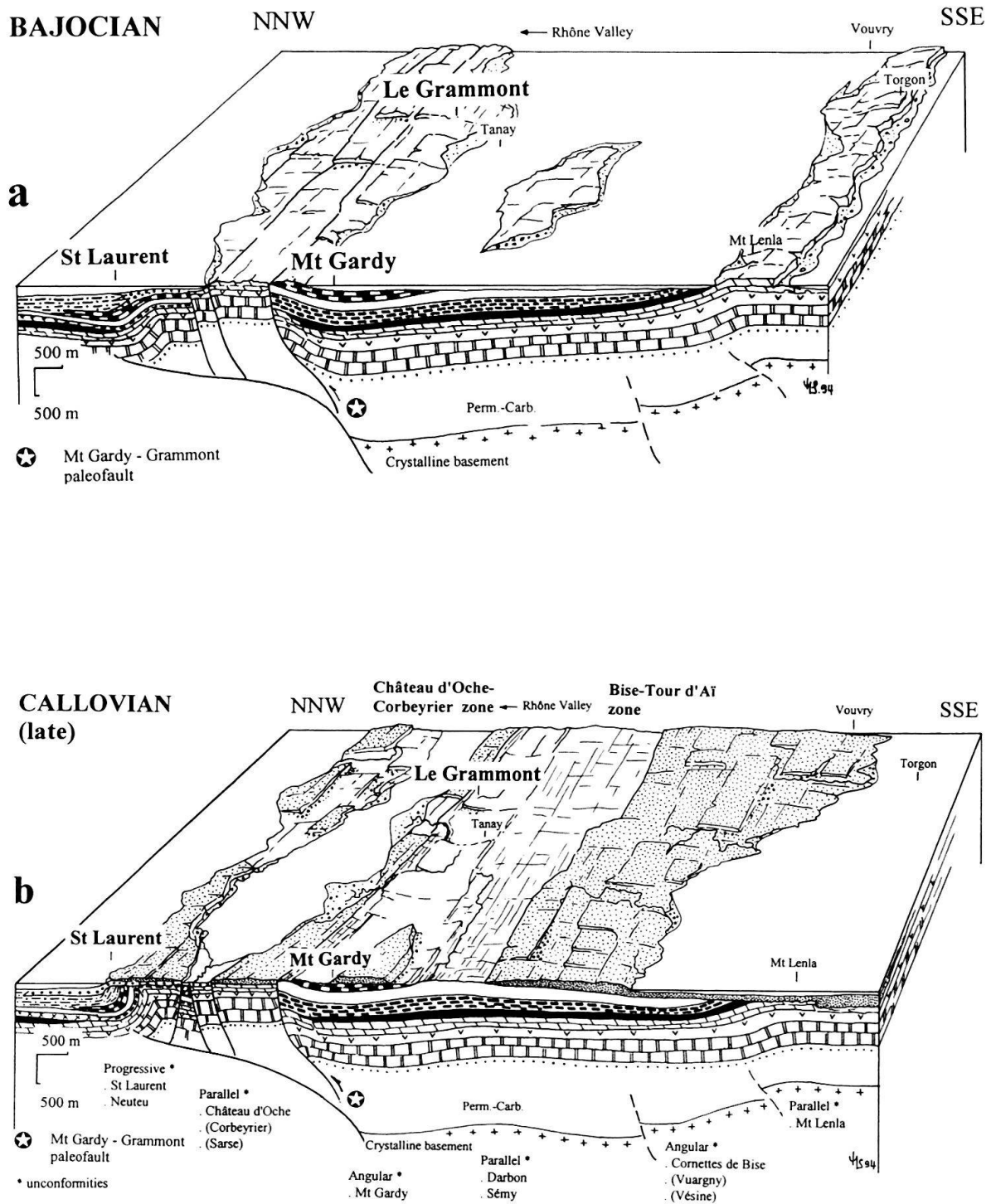
Fig. 9a. Block diagram of the studied area (eastern Chablais) during Bajocian times, showing relations between paleostructures at depth and superficial relief evolution. b. Block diagram of the same area during Late Callovian times. Compressive movements trigger the uplift of the central part of the Briançonnais carbonate platform (Bise-Tour d'Ai zone) with emersion and erosion in the Château d'Oche zone. The Middle Jurassic Mytilus Formation (stippled) is strongly eroded by karstic dissolution. Along the northern coast, rivers brought coarse sediments coming from Middle Liassic outcrops of the Bise-Tour d'Ai zone. This paleotectonic event has been previously called the Callovo-Oxfordian phase by Septfontaine (1984) Block diagram b is slightly enlarged compared to a. Legend of lithologic symbols on figures 2 and 8.
