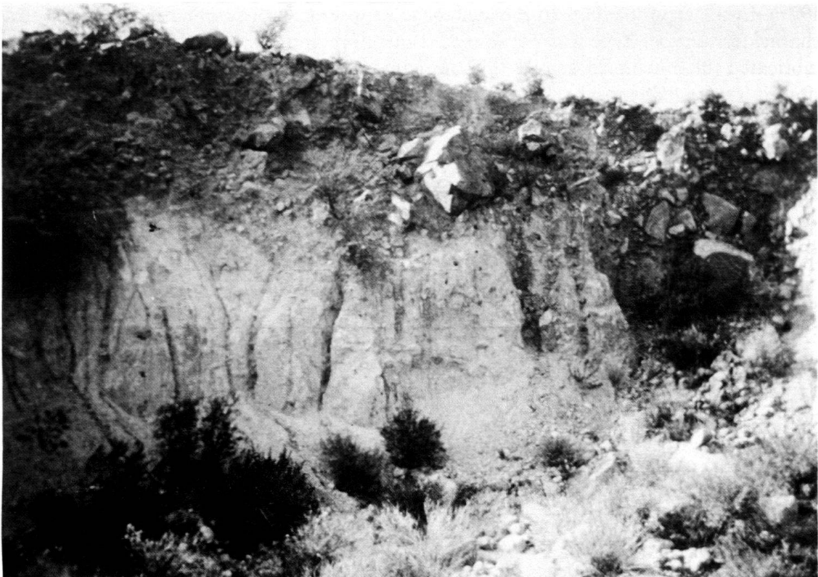
Fig. 6. Inverse grading at the Loma de la Aspereza rock-avalanche.
