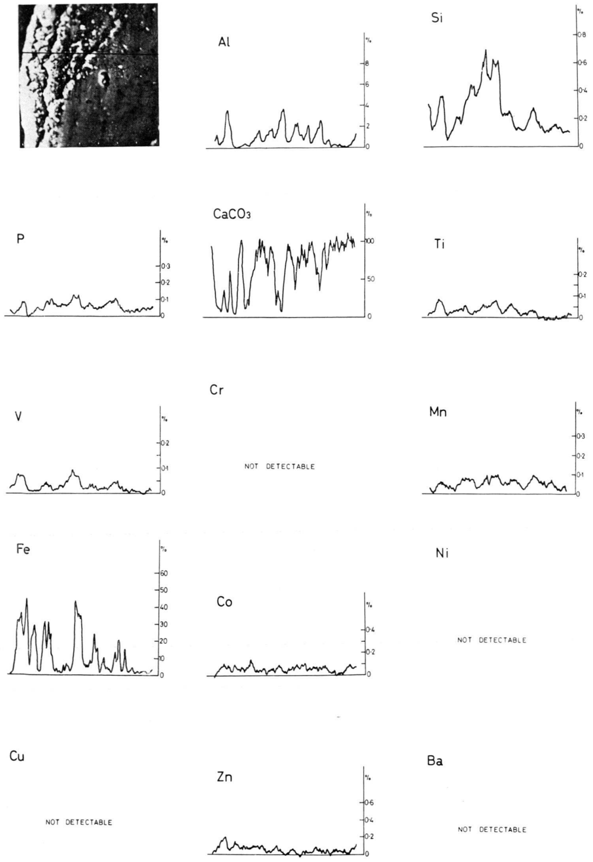
Fig.18. Electron-probe microanalysis of an iron oolite from the Bathonian Twinhoe Beds of Somerset, England. Length of scan line = 375 \mu .
