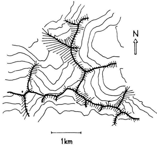
Fig. 7. Plan view of pyramidal peaks with three ledges. Hühnerstock, 3307 m, Aar-Massiv, Swiss Alps (Schematic).
