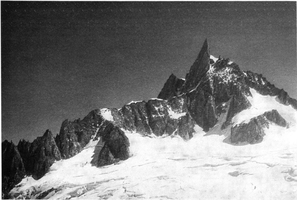
Fig. 11. Ledge of a pyramidal peak with tensional cracks and fissures, split into individual blocks and towers. Aiguille du Géant, 4013 m, Mont-Blanc, France.
