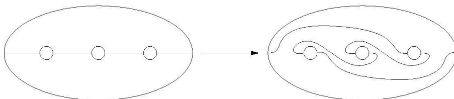
Figure 6. The braid relation in \overline{\text{Mod}}(\overline{S}) .
