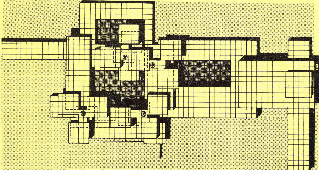
2 Grundriß 2. Stock 1:1000
