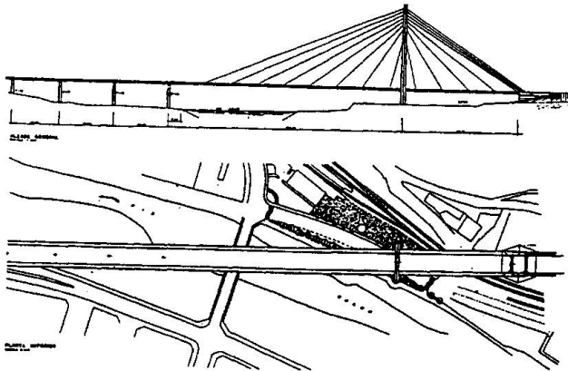
Figure 1. Sama de Langreo Bridge in Spain. Elevation
