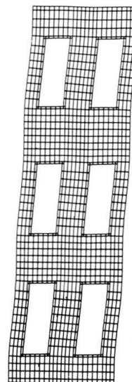
FIGURE 12 - DEFORMED SHAPE OF EXTERIOR WALL
