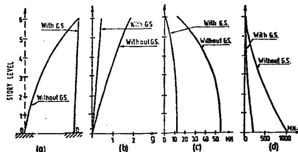
Fig. 4. The Endul building in Managua, Nicaragua. Design values, North-South direction, with and without the GAPEC SYSTEM (a) 1st predominant mode shape (b) acceleration-response; (c) shears; (d) overturning moments.
