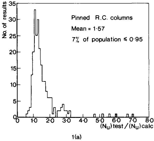
FIGURE 1 (N_U)_{TEST}/(N_U)_{CALC} USING ADDITIONAL MOMENT EXPRESSION FOR R.C. SECTIONS
