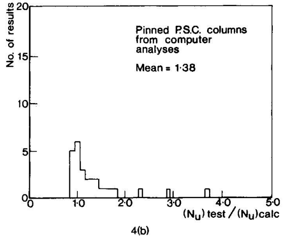
FIGURE 4 (N_U)_{TEST}/(N_U)_{CALC} USING MODIFIED ADDITIONAL MOMENT EXPRESSION
