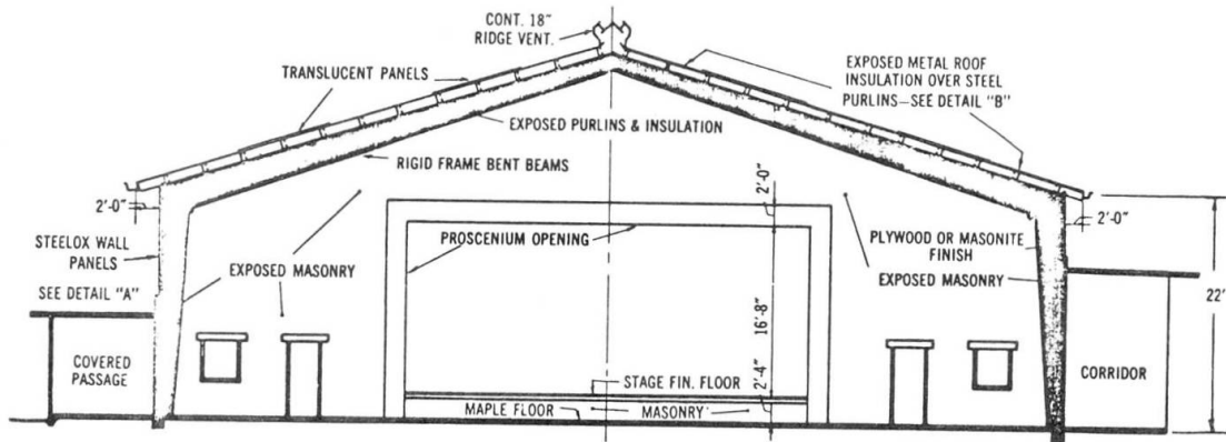
Cross Section—Gymnasium-Auditorium
