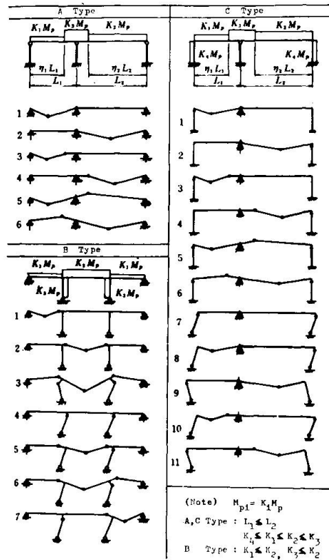
Collapse mechanisms
