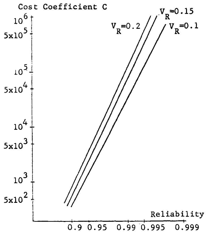
FIG. 3 COST COEFFICIENT VS. OPTIMAL ELEMENT RELIABILITY--PARALLEL SYSTEM
