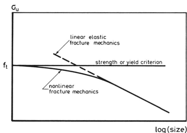
Fig. 9 Size effect according to various theories.
