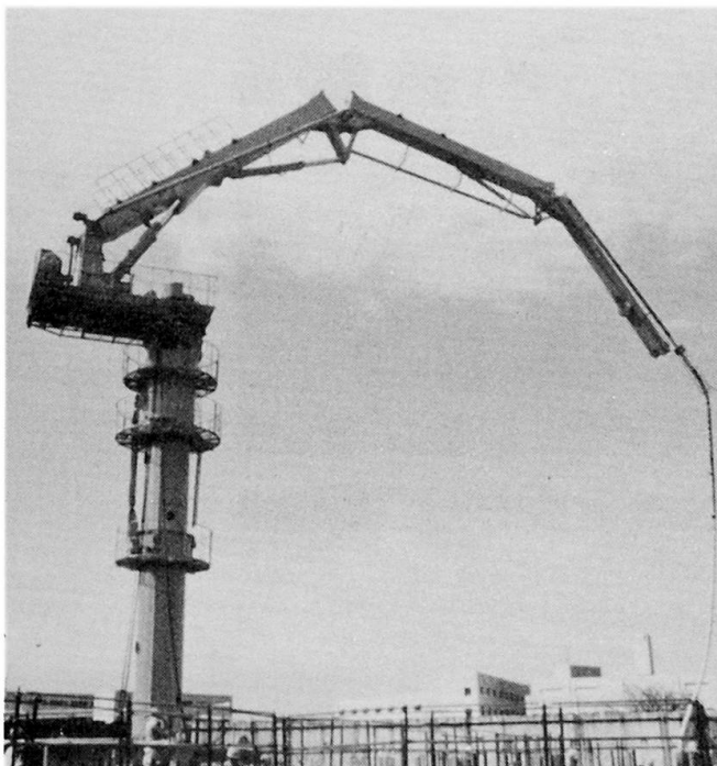
Photo 4 Con-disk crane
