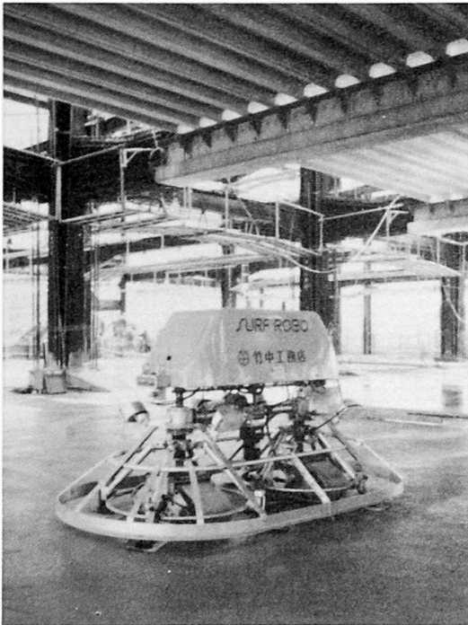
Photo 6 Surf robot
