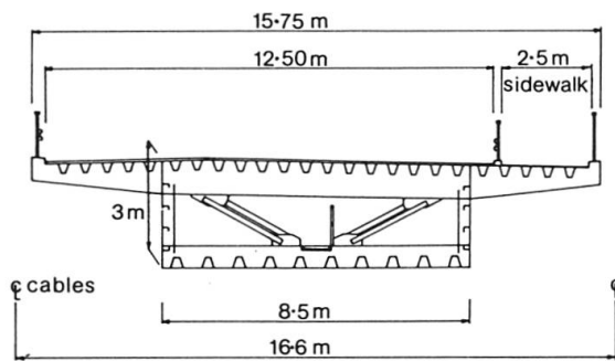
Fig. 1. Cross sections
